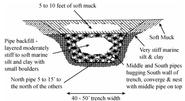
Fig. 6 Typical pipe trench conditions found during investigation.
