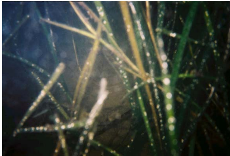
Typical Eelgrass Bed in New England (Photo 1)
